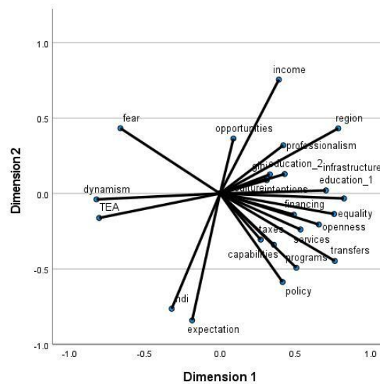
Figure 6: Component Loadings (Growth 2010-2020) Source: Compiled by the authors.
