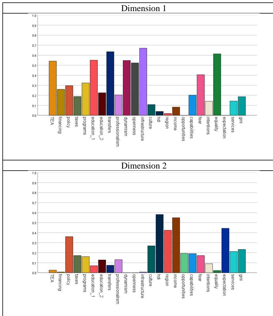
Figure 4: Variance Accounted for in the First Two Dimensions (Growth 2010-2020) Source: Compiled by the authors.
