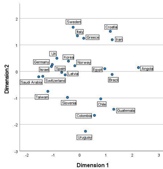
Figure 2: Object Points Labelled by Country (Year 2020) Source: Compiled by the authors.
