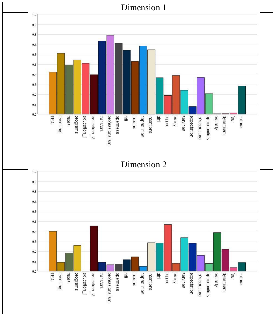
Figure 1: Variance Accounted for in the First Two Dimensions (Year 2020) Source: Compiled by the authors.
