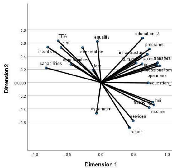
Figure 3: Component Loadings (Year 2020) Source: Compiled by the authors.
