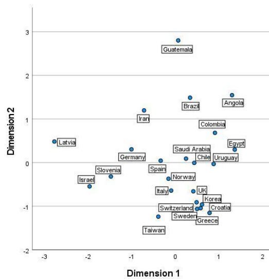
Figure 5: Object Points Labelled by Country (Growth 2010-2020) Source: Compiled by the authors.
